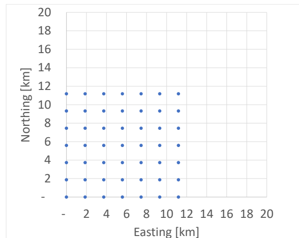
Figure 2: Modelled wind farm layout with 8 MW/km 2 build-out density (run ID 6).
