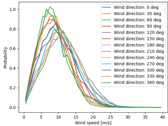
Figure 9 Annual distribution of wind speeds at 110m above mean sea level (AMSL).
